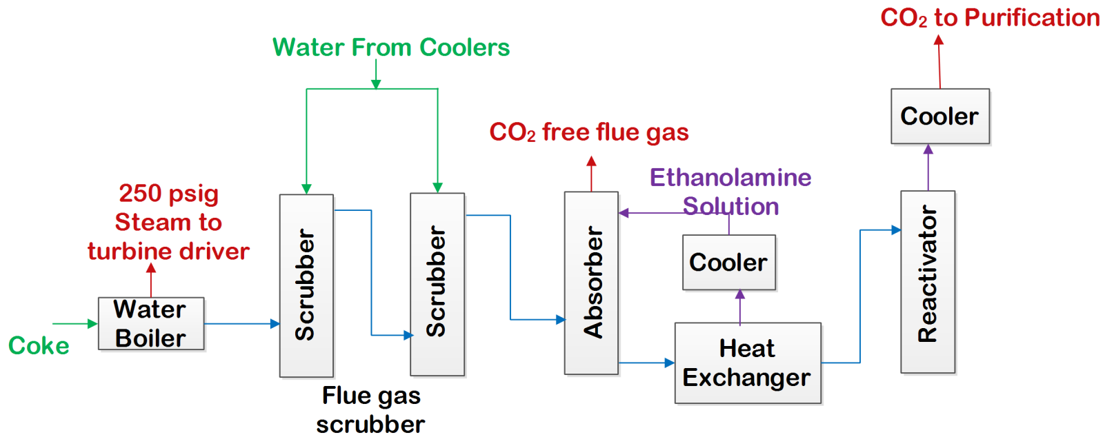
Figure: Manufacture of Carbon dioxide by Coke
